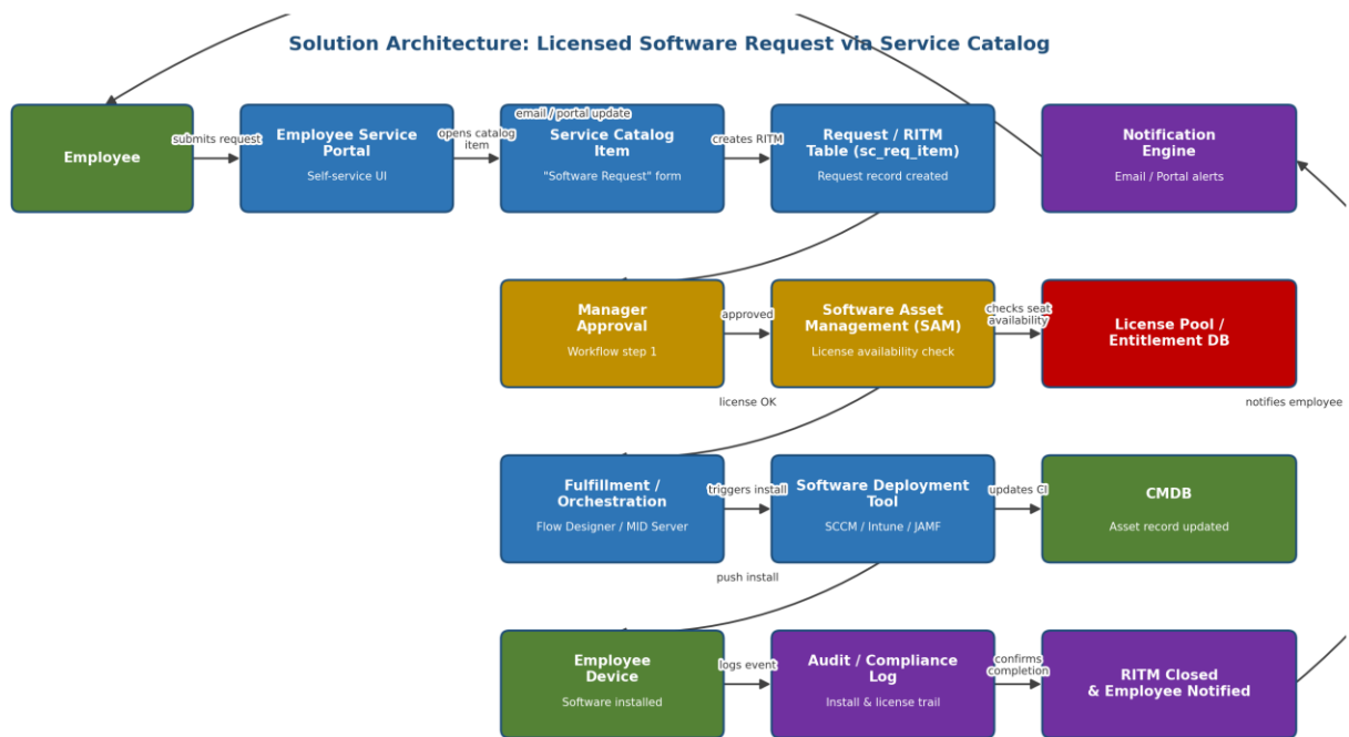
Figure 1: Architecture and data flow for licensed software requests submitted through the Service Catalog
